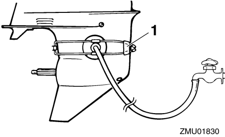
1. Flushing attachment
