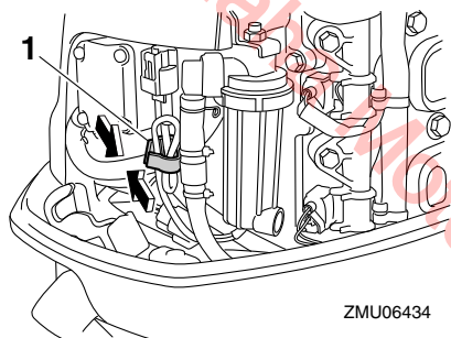
1. Holder
